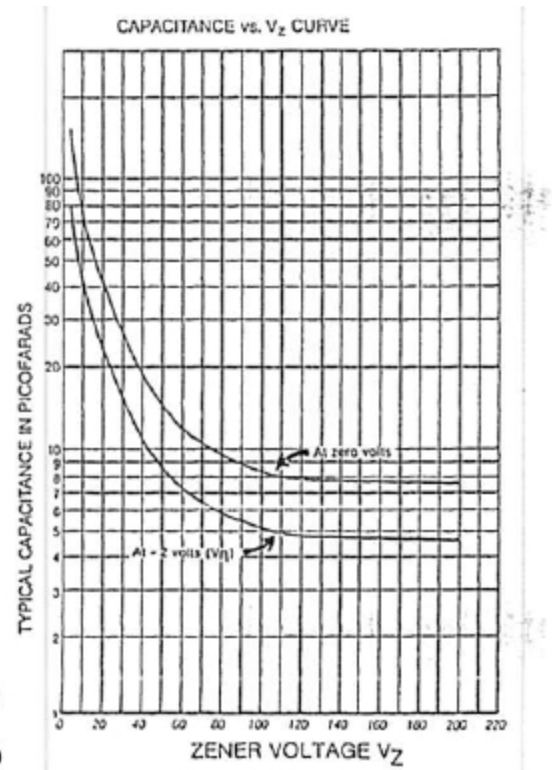
FIGURE 2 CAPACITANCE vs. ZENER VOLTAGE (TYPICAL)
