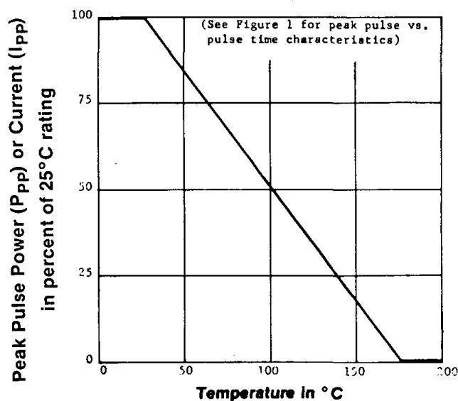
FIGURE 3 Derating Curve
