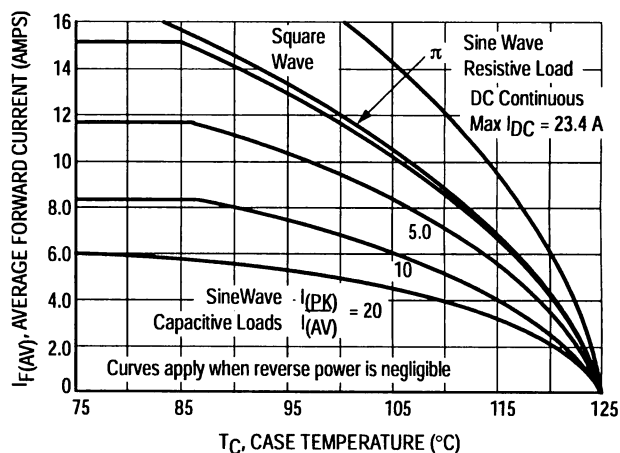
Figure 7. Current Derating
