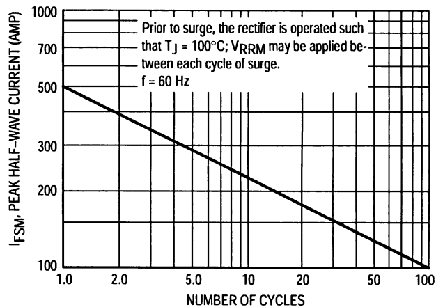
Figure 6. Maximum Surge Capability
