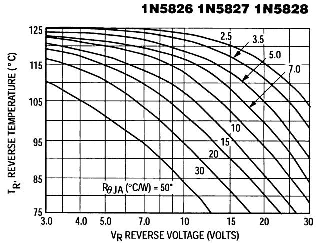
Figure 2. Maximum Reference Temperature – 1N5827
