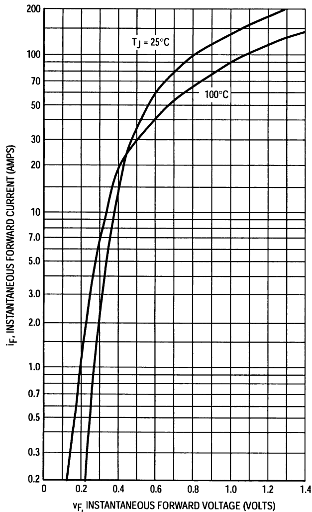
Figure 5. Typical Forward Voltage
