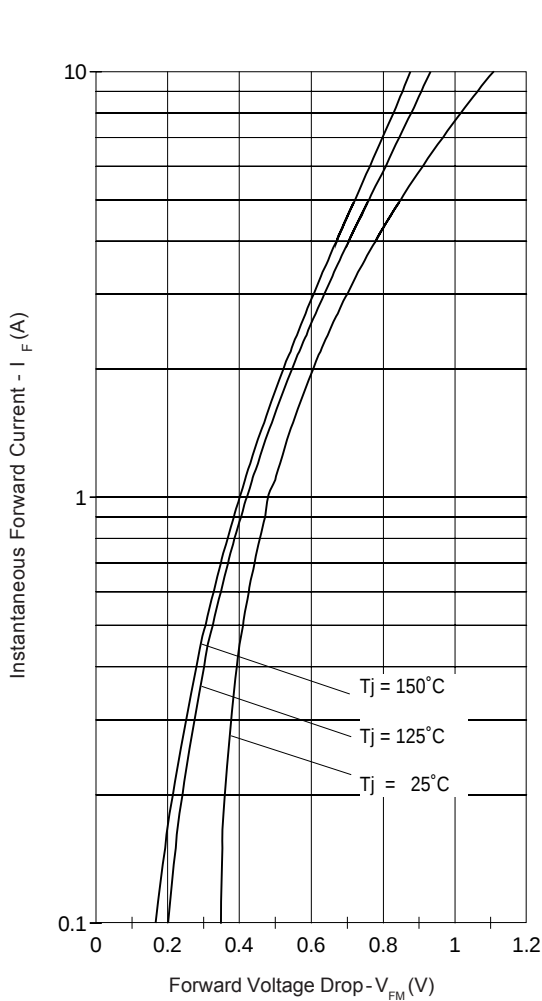
Fig. 1 - Typ. Forward Voltage Drop Characteristics
