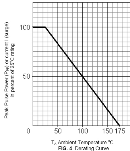
FIG. 4 Derating Curve
