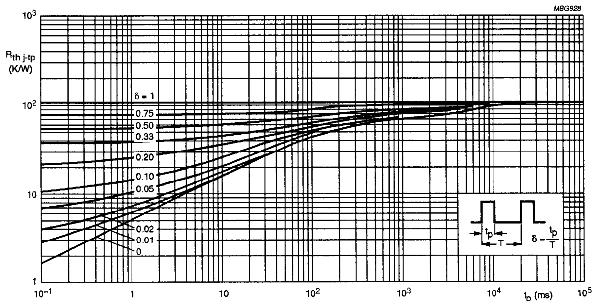
Fig.2 Thermal resistance from junction to tie-point; lead length 4 mm.
