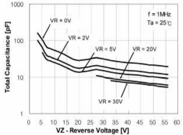
Figure 2. Total Capacitance
