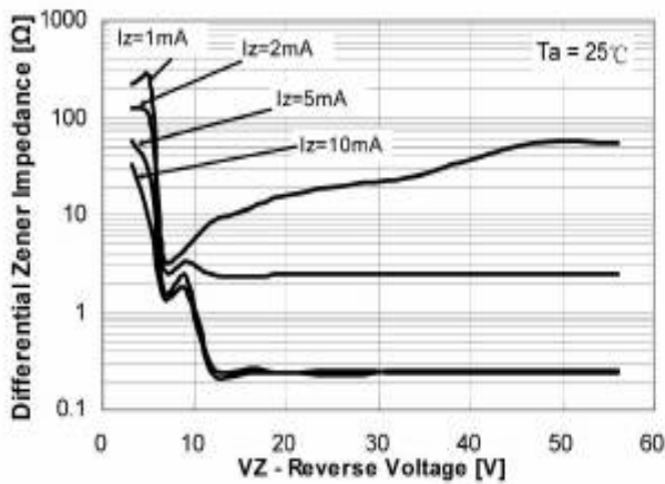
Figure 3. Differential Impedance vs. Zener Voltage
