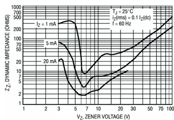
Figure 3. Effect of zener voltage on zener impedance
