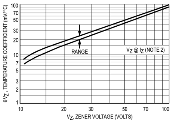
Figure 3. Temperature coefficients
