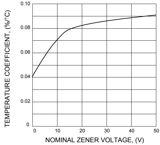
FIG.2 - ZENER VOLTAGE TEMPERATURE COEFFICIENT VS. ZENER VOLTAGE
