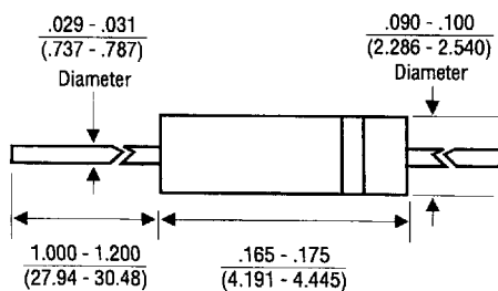
DO-41
