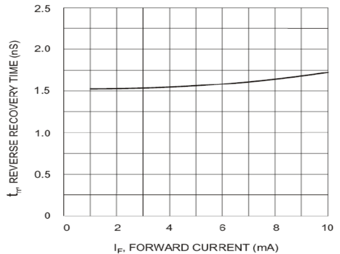
Fig. 4 Reverse Recovery Time vs. Forward Current
