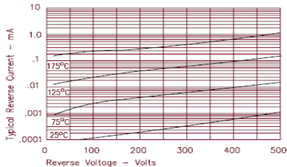
FIGURE 2 TYPICAL REVERSE CHARACTERISTICS
