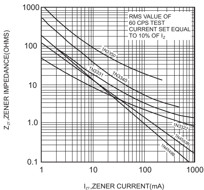
Fig. 2 - Typical Zener Impedance Vs Zener Current
