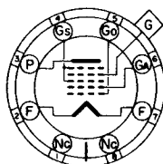
SMALL 8 PIN OCTAL BASE 1C7G
