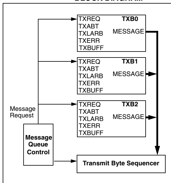
FIGURE 19-2: TRANSMIT BUFFER BLOCK DIAGRAM
