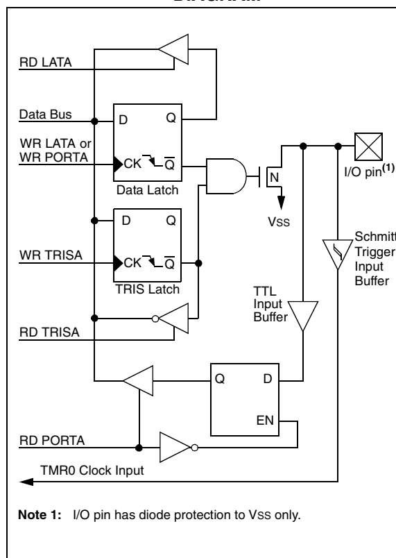
FIGURE 9-2: RA4/T0CKI PIN BLOCK DIAGRAM
