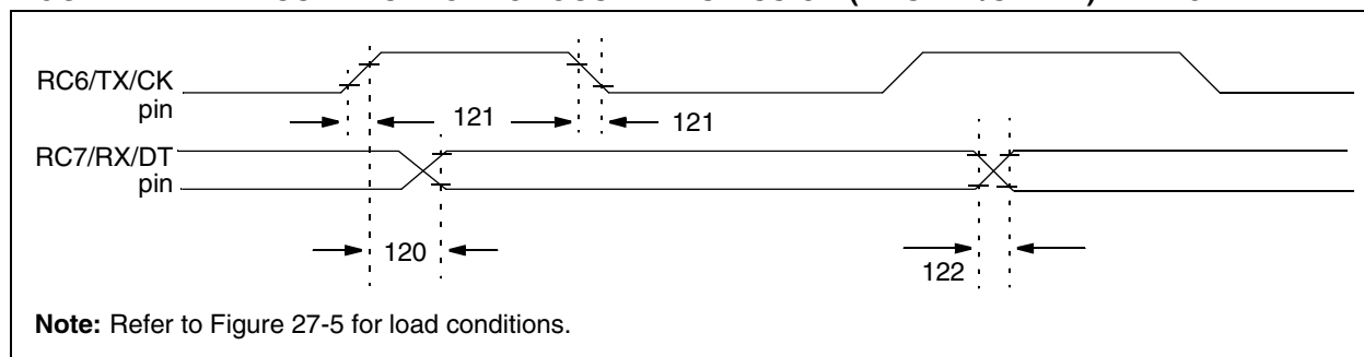
FIGURE 27-21: USART SYNCHRONOUS TRANSMISSION (MASTER/SLAVE) TIMING
