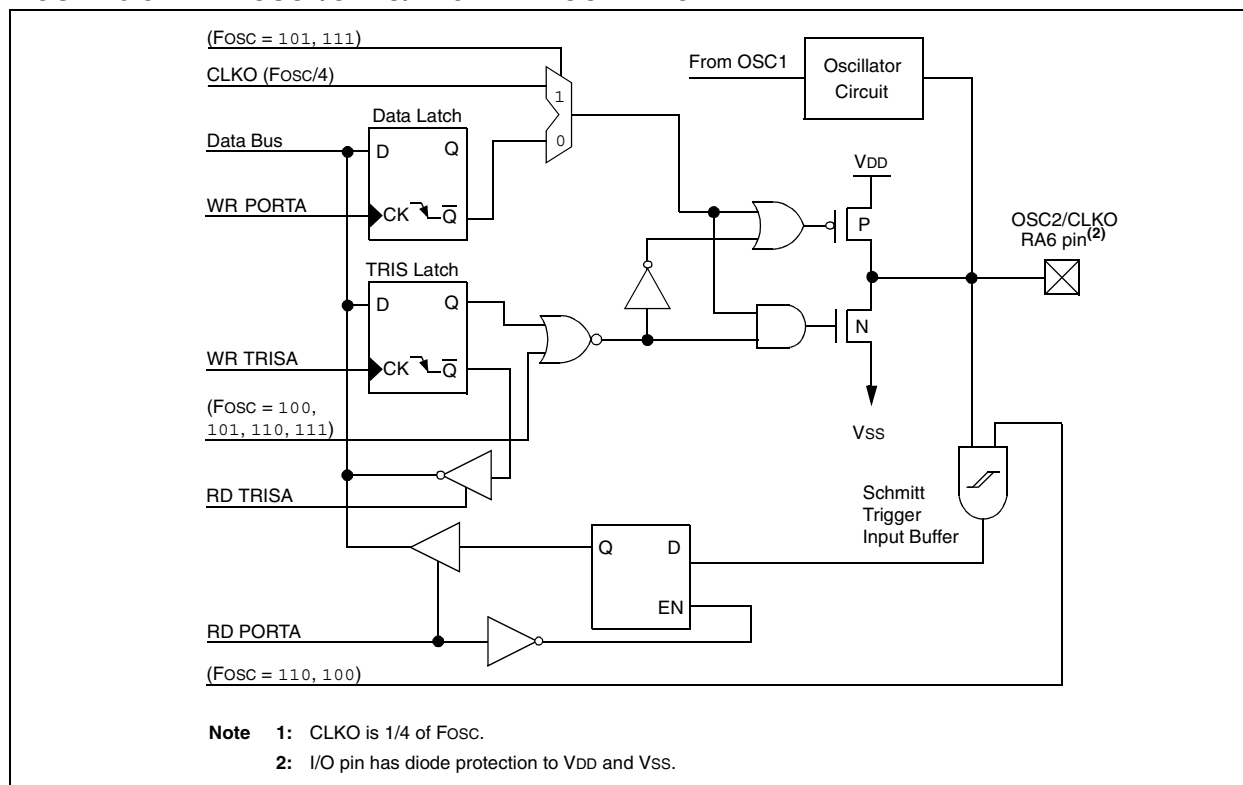
FIGURE 9-3: OSC2/CLKO/RA6 PIN BLOCK DIAGRAM
