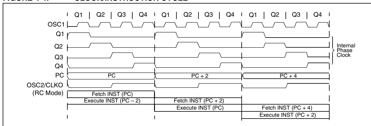
FIGURE 4-4: CLOCK/INSTRUCTION CYCLE
