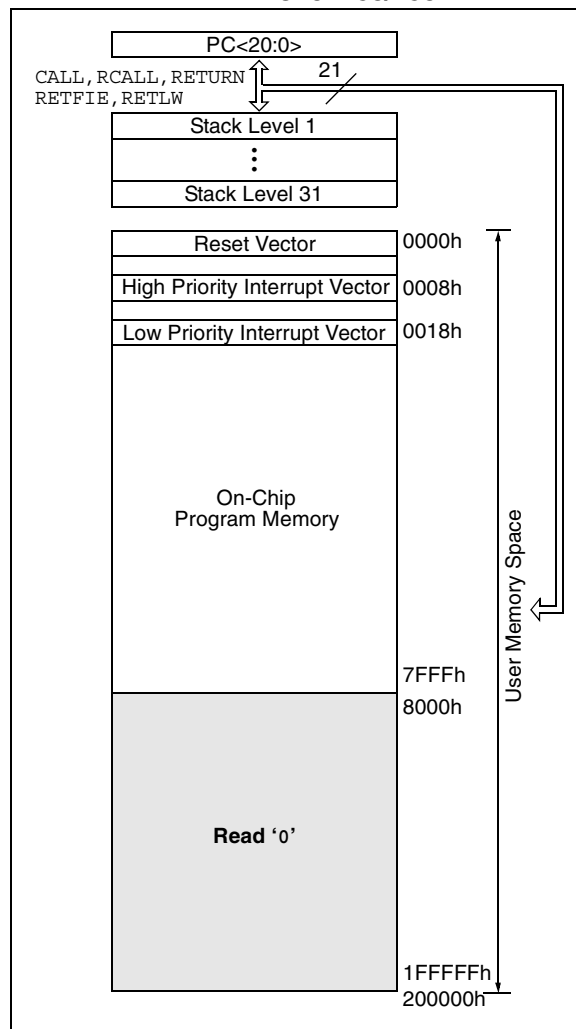
FIGURE 4-2: PROGRAM MEMORY MAP AND STACK FOR PIC18F258/458
