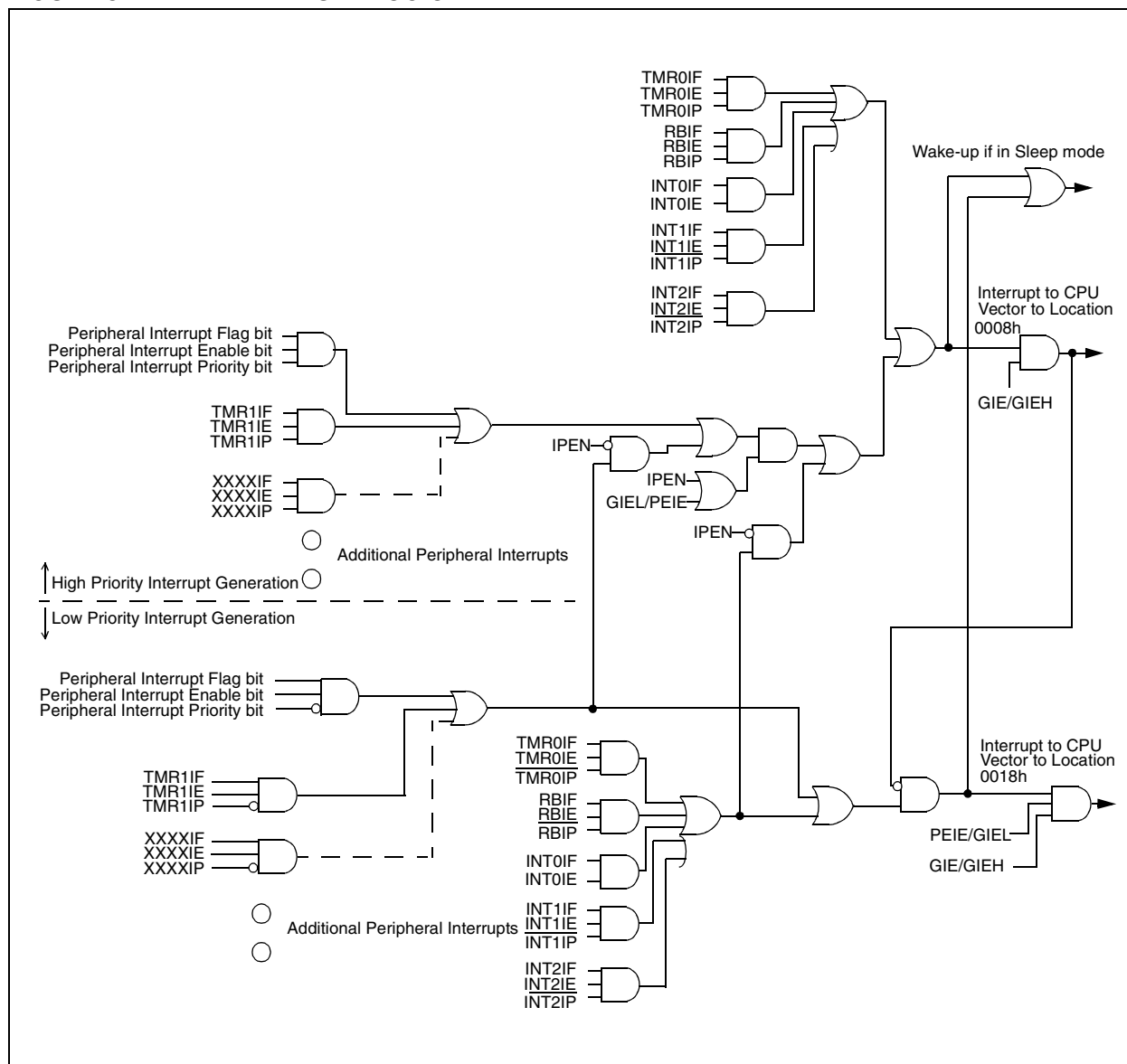
FIGURE 8-1: INTERRUPT LOGIC
