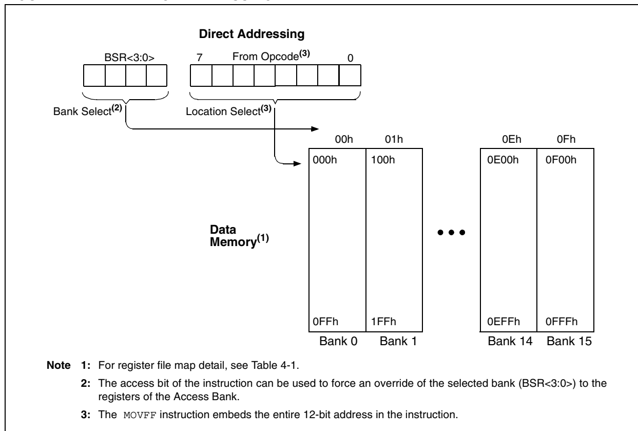
FIGURE 4-7: DIRECT ADDRESSING
