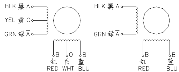
UNI-POLAR(6 LEADS)
