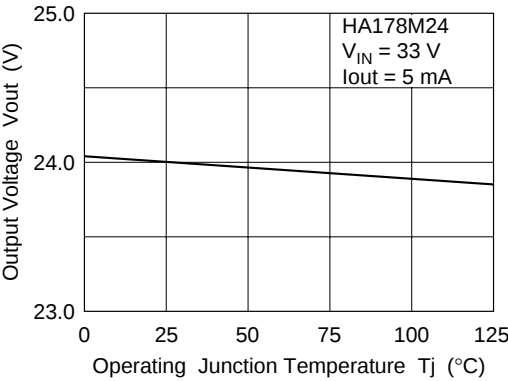
Output Voltage vs. Operating Junction Temperature (3)
