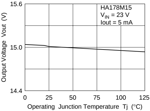
Output Voltage vs. Operating Junction Temperature (2)
