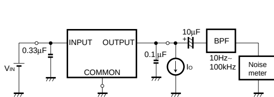
Fig. 3 Measurement circuit for output noise voltage
