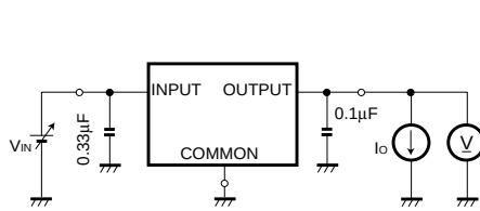
Fig. 1 Measurement circuit for output voltage, input stability, load regulation, temperature coefficient of output voltage
