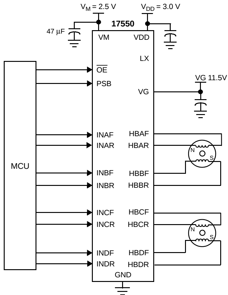
Figure 7. Typical 17550 Application - No Internal DC-DC Used
