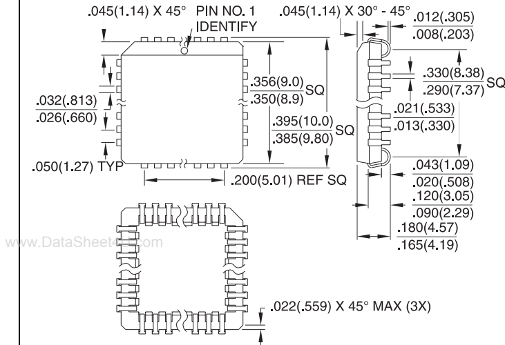
20J , 20-lead, Plastic J-Leaded Chip Carrier (PLCC) Dimensions in Inches and (Millimeters) JEDEC STANDARD MS-018 AA
