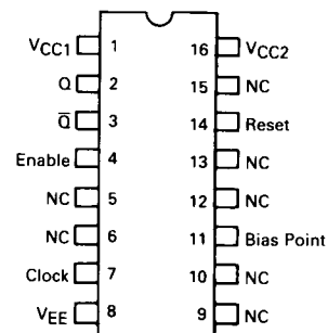
PIN ASSIGNMENT
