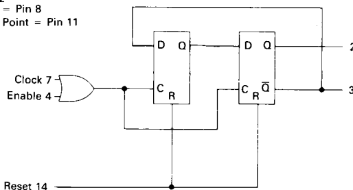
LOGIC DIAGRAM
