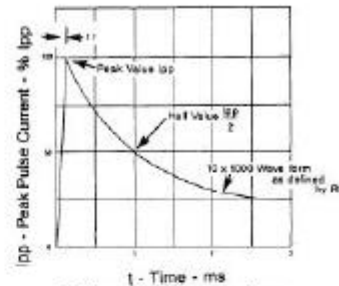
FIGURE 2 Pulse Waveform
