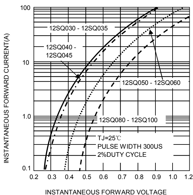
FIG.4-TYPICAL FORWARD CHARACTERISTICS
