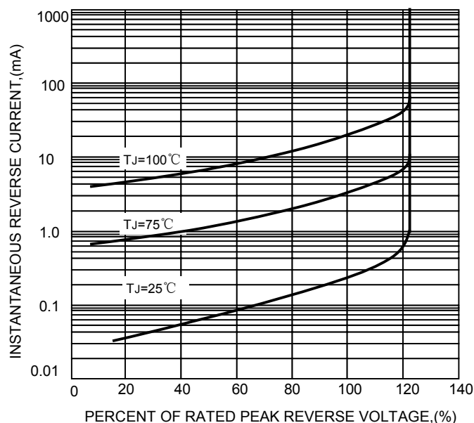
FIG.3-TYPICAL REVER CHARACTERISTICS
