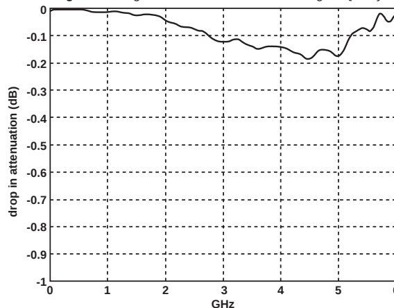
Figure 2. SurgX® induced interference with Signal Quality
