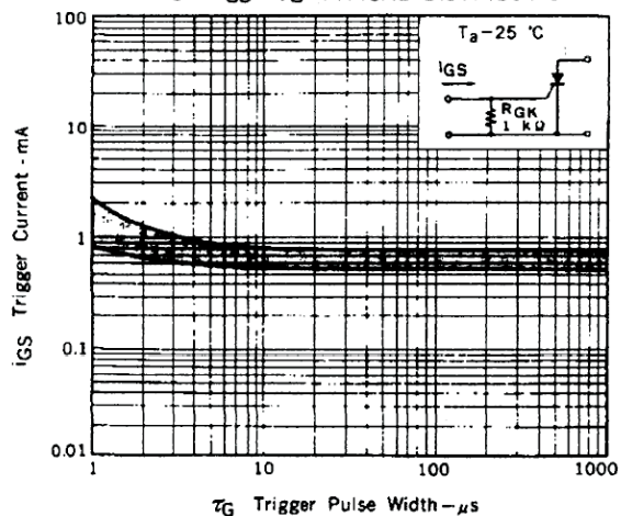
Fig. 7 I_{GS} - \tau_G TYPICAL DISTRIBUTION
