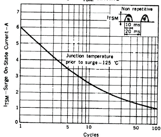
Fig. 2 I_{TSM} RATING
